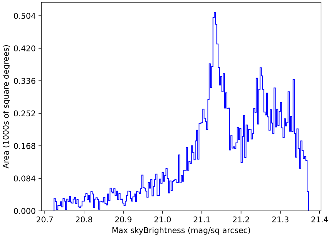
too_elab_r64_d3_griz_v3.4_10yrs Yr 1 r band: Max skyBrightness
