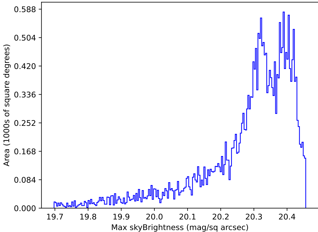
too_elab_r64_d3_griz_v3.4_10yrs Yr 1 i band: Max skyBrightness
