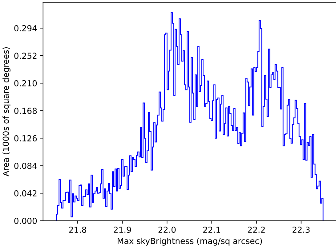
too_elab_r64_d3_griz_v3.4_10yrs Yr 1 g band: Max skyBrightness
