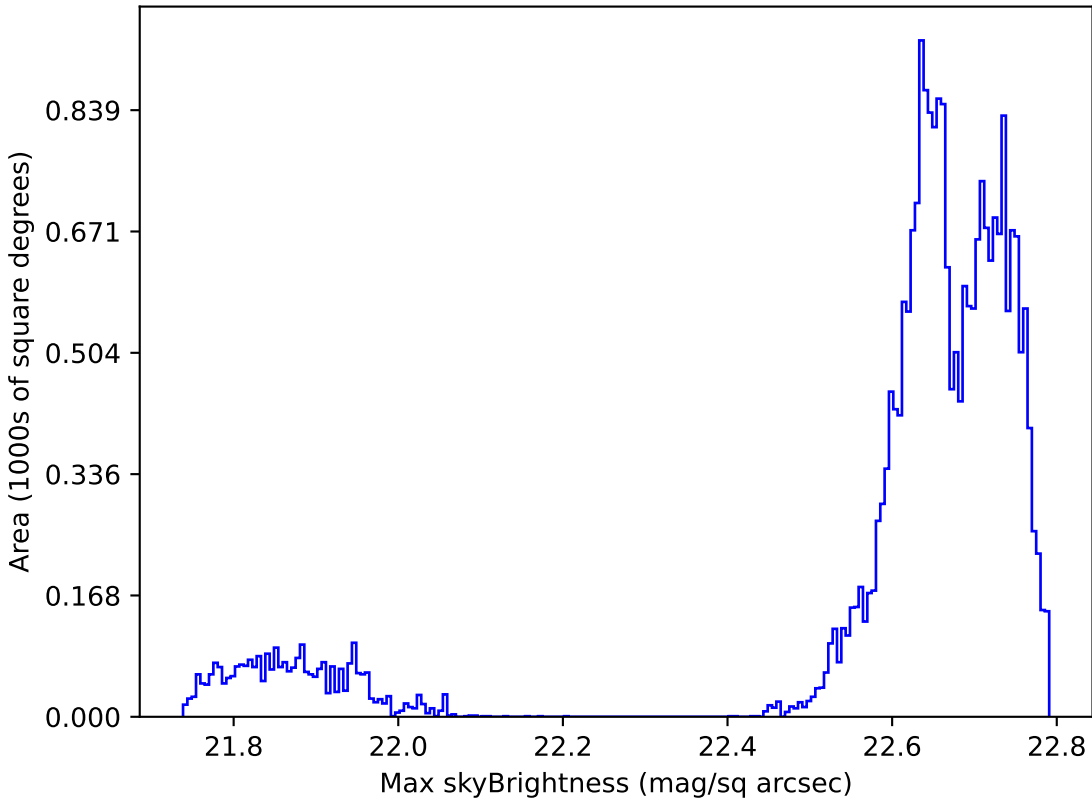
too_elab_r64_d3_griz_v3.4_10yrs Yr 1 all bands: Max skyBrightness
