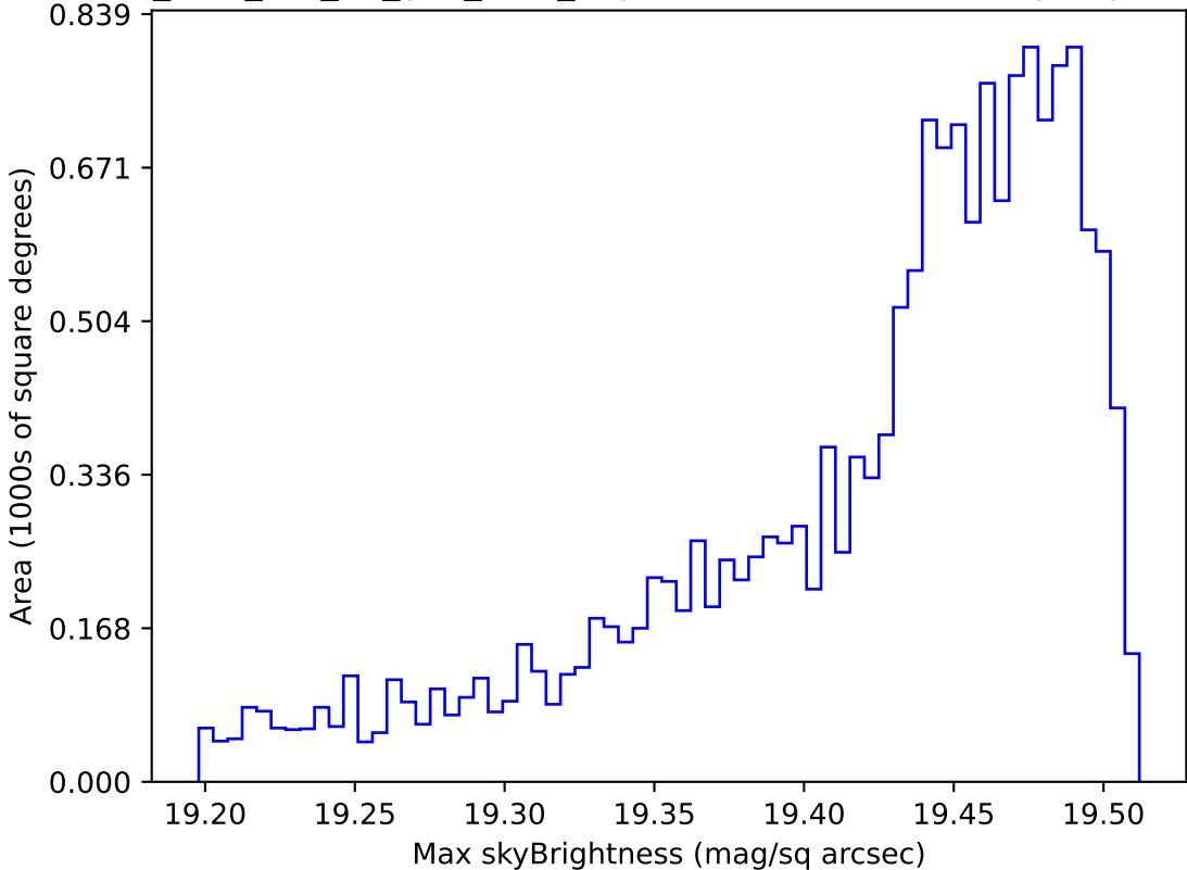
too_elab_r64_d3_griz_v3.4_10yrs WFD z band: Max skyBrightness
