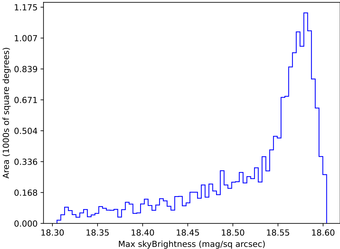
too_elab_r64_d3_griz_v3.4_10yrs WFD y band: Max skyBrightness
