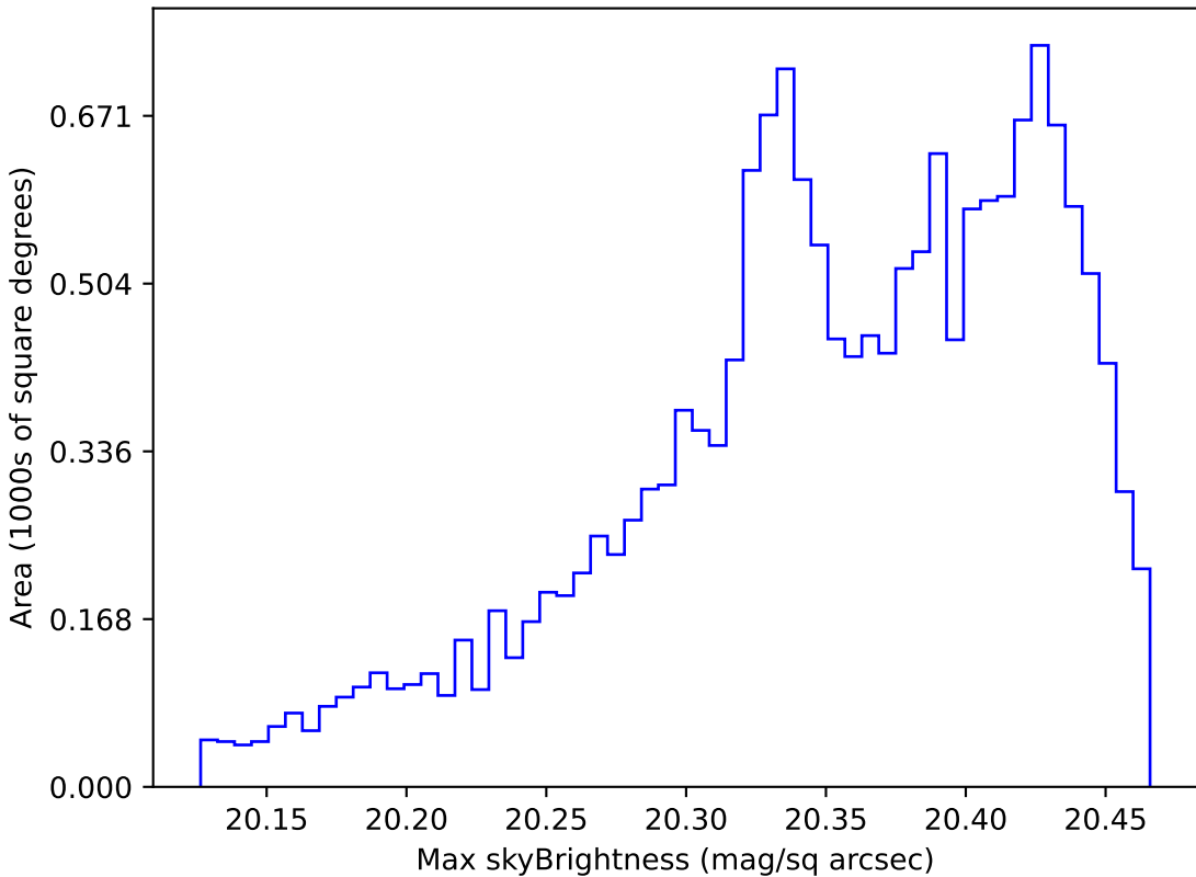
too_elab_r64_d3_griz_v3.4_10yrs WFD i band: Max skyBrightness
