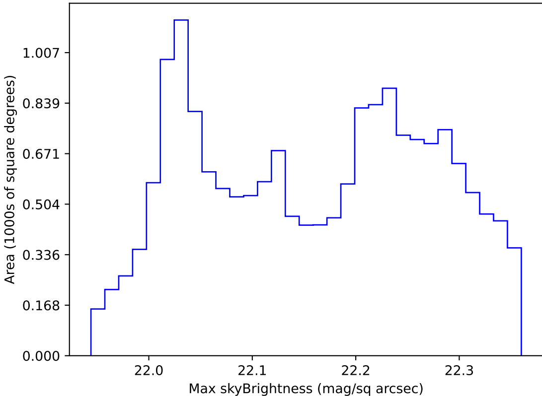
too_elab_r64_d3_griz_v3.4_10yrs WFD g band: Max skyBrightness
