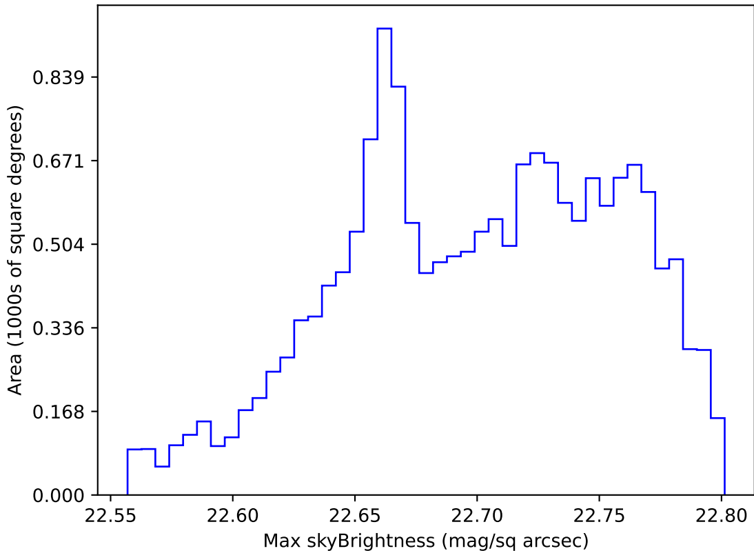
too_elab_r64_d3_griz_v3.4_10yrs WFD all bands: Max skyBrightness
