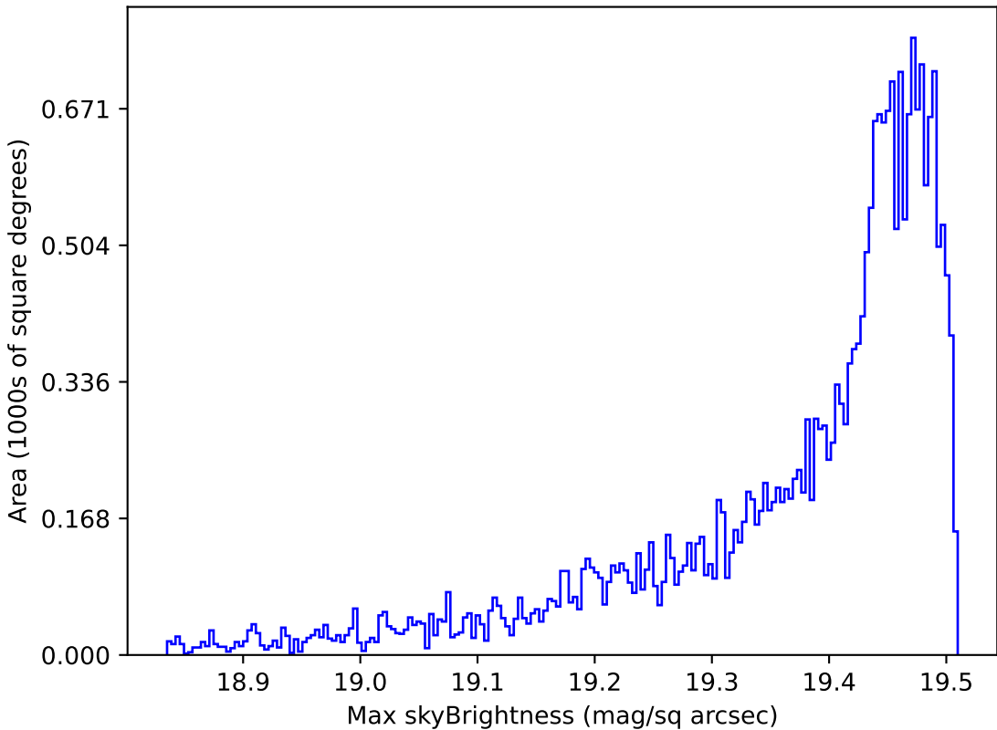
too_elab_r64_d3_griz_v3.4_10yrs All sky z band: Max skyBrightness
