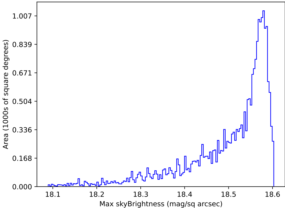
too_elab_r64_d3_griz_v3.4_10yrs All sky y band: Max skyBrightness
