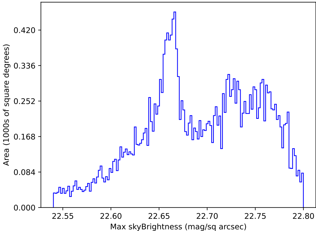
too_elab_r64_d3_griz_v3.4_10yrs All sky u band: Max skyBrightness
