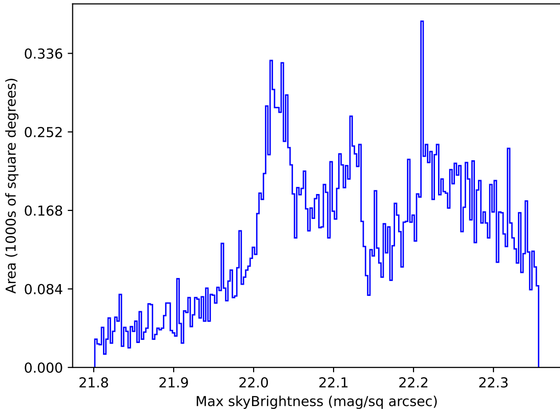
too_elab_r64_d3_griz_v3.4_10yrs All sky g band: Max skyBrightness
