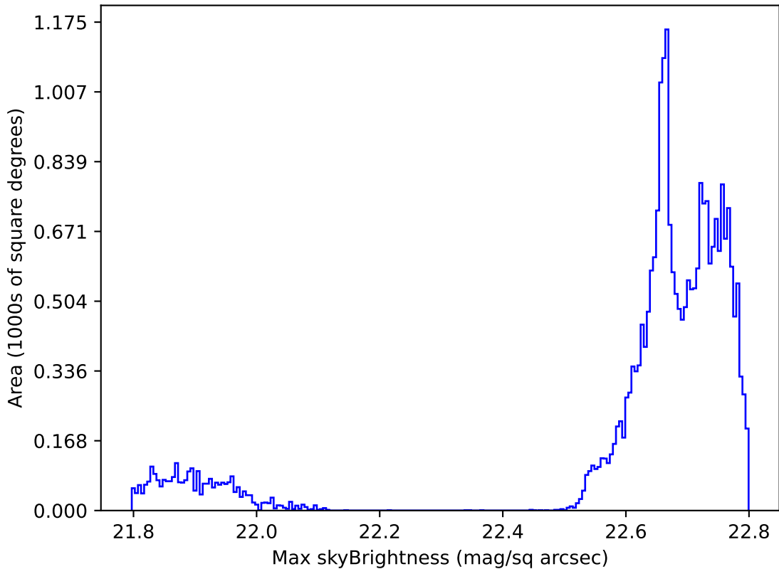
too_elab_r64_d3_griz_v3.4_10yrs All sky all bands: Max skyBrightness
