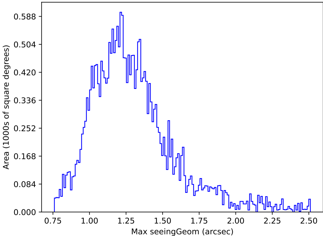
too_elab_r64_d3_griz_v3.4_10yrs Yr 1 z band: Max seeingGeom
