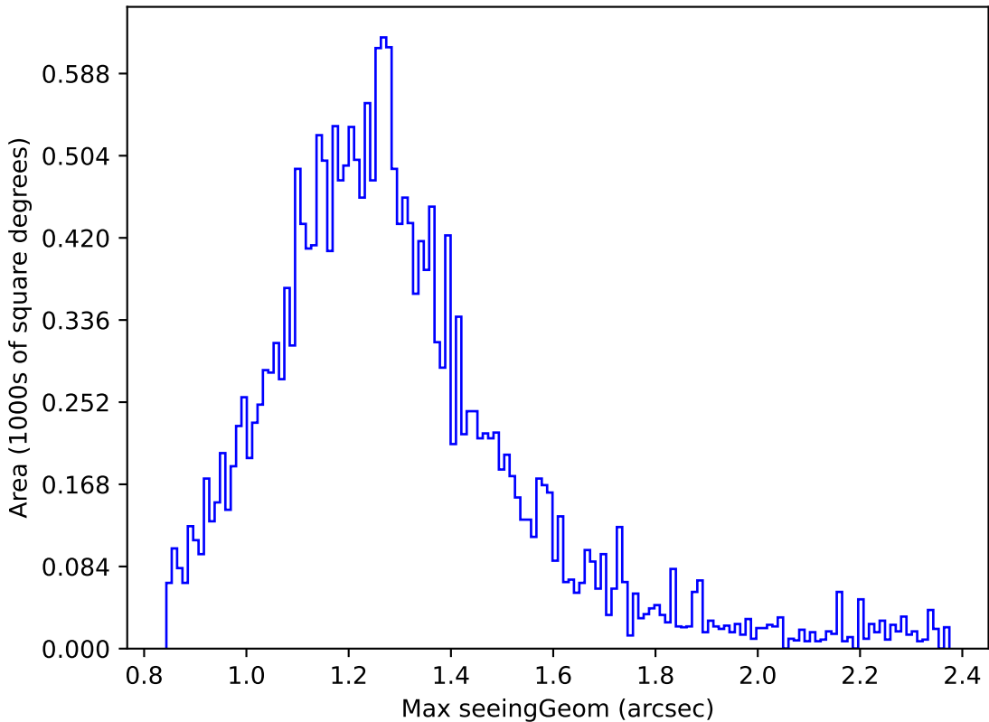
too_elab_r64_d3_griz_v3.4_10yrs Yr 1 y band: Max seeingGeom
