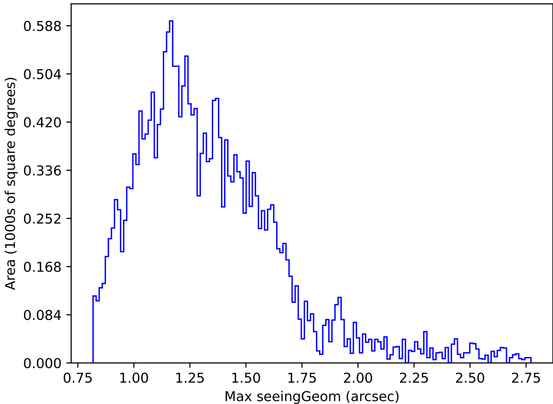
too_elab_r64_d3_griz_v3.4_10yrs Yr 1 u band: Max seeingGeom
