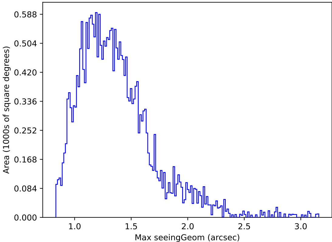
too_elab_r64_d3_griz_v3.4_10yrs Yr 1 g band: Max seeingGeom
