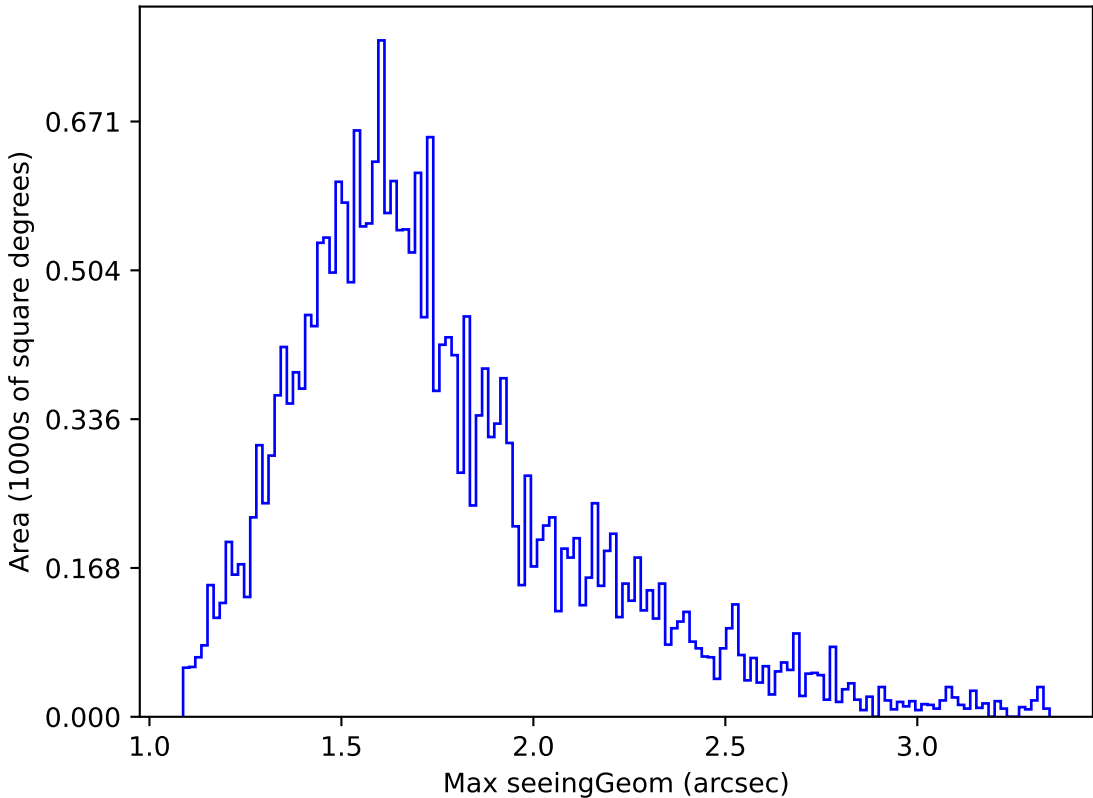
too_elab_r64_d3_griz_v3.4_10yrs Yr 1 all bands: Max seeingGeom
