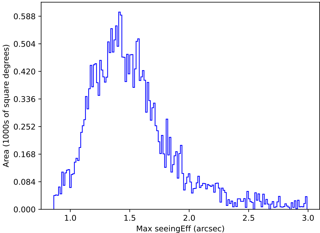
too_elab_r64_d3_griz_v3.4_10yrs Yr 1 z band: Max seeingEff
