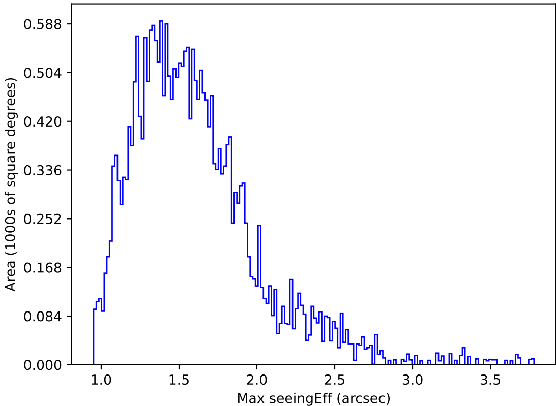
too_elab_r64_d3_griz_v3.4_10yrs Yr 1 g band: Max seeingEff
