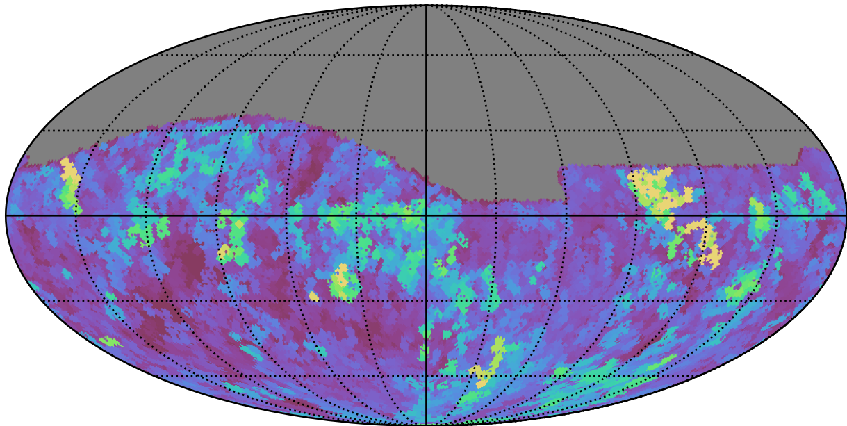
too_elab_r64_d3_griz_v3.4_10yrs Yr 1 all bands: Max seeingEff
