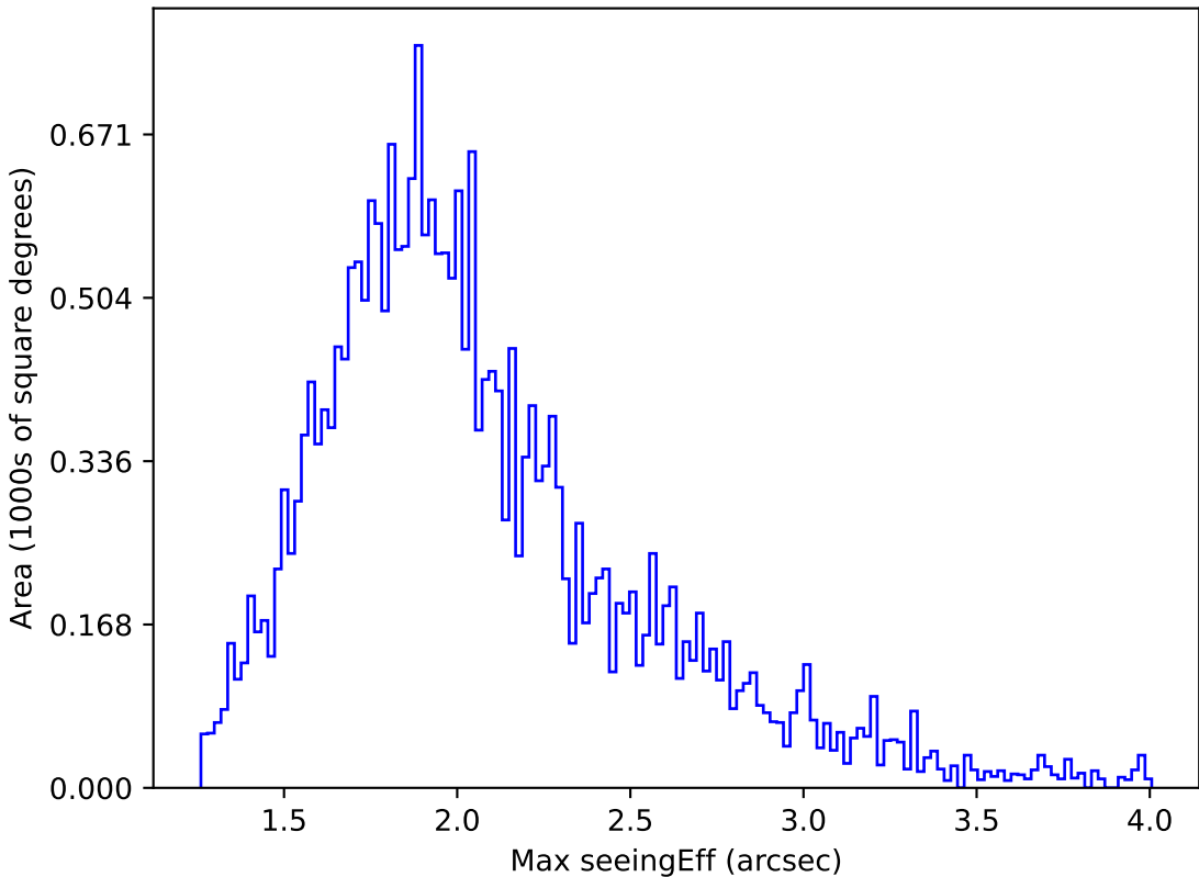
too_elab_r64_d3_griz_v3.4_10yrs Yr 1 all bands: Max seeingEff
