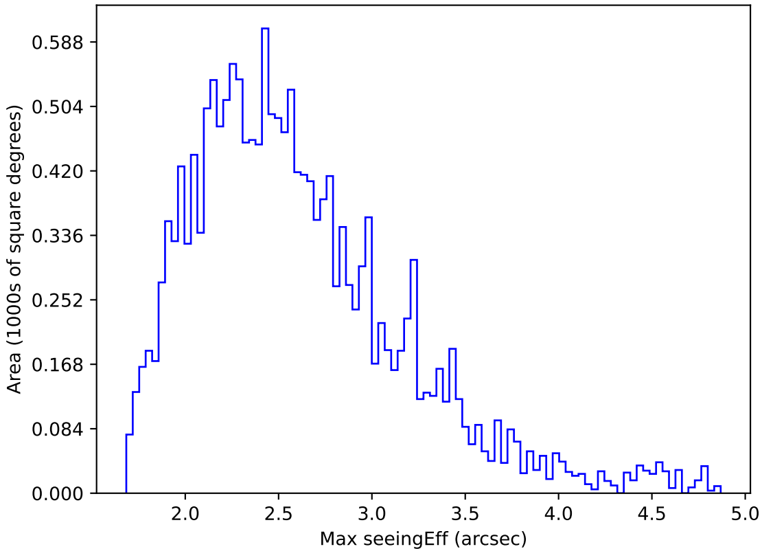
too_elab_r64_d3_griz_v3.4_10yrs WFD z band: Max seeingEff
