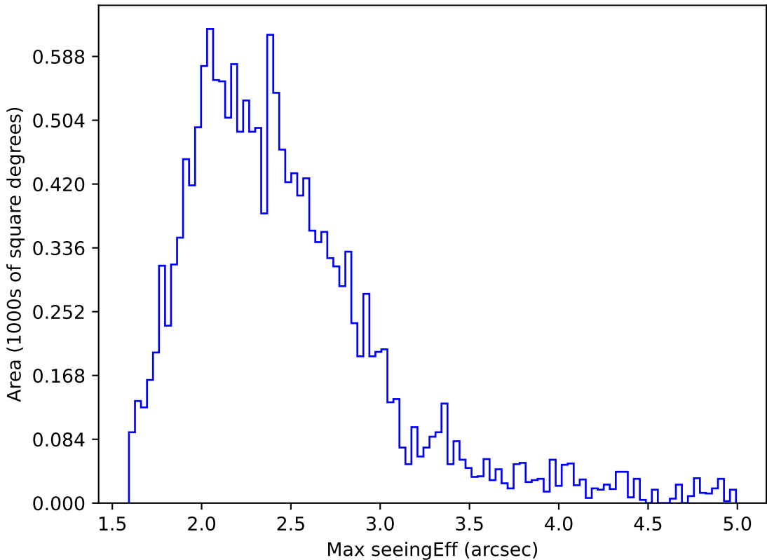
too_elab_r64_d3_griz_v3.4_10yrs WFD y band: Max seeingEff
