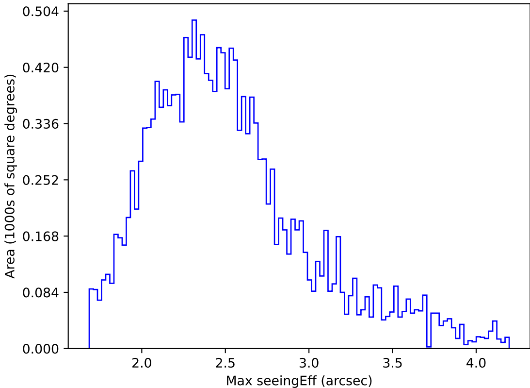
too_elab_r64_d3_griz_v3.4_10yrs WFD g band: Max seeingEff
