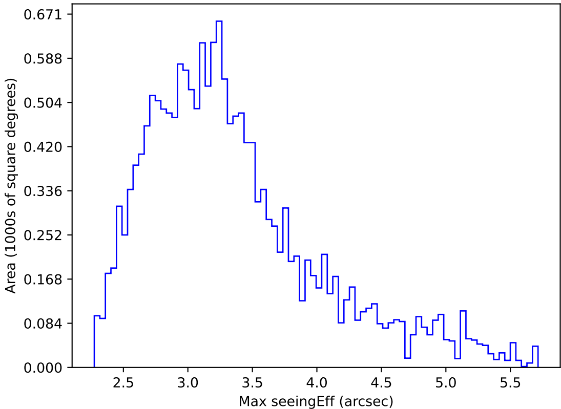
too_elab_r64_d3_griz_v3.4_10yrs WFD all bands: Max seeingEff
