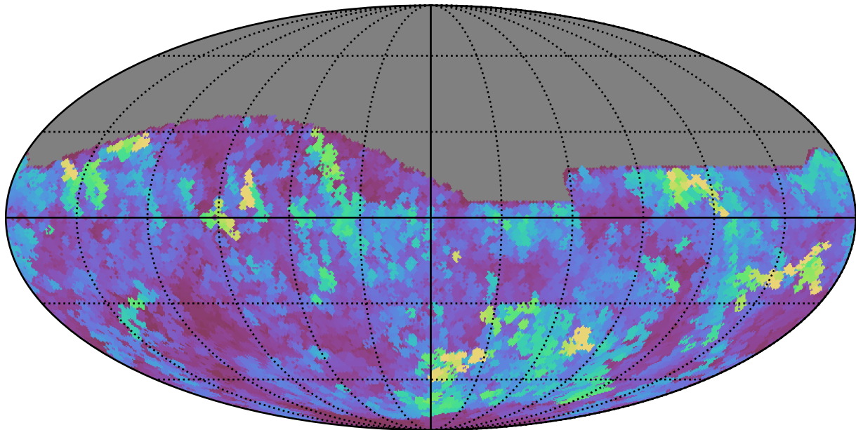
too_elab_r64_d3_griz_v3.4_10yrs All sky z band: Max seeingEff
