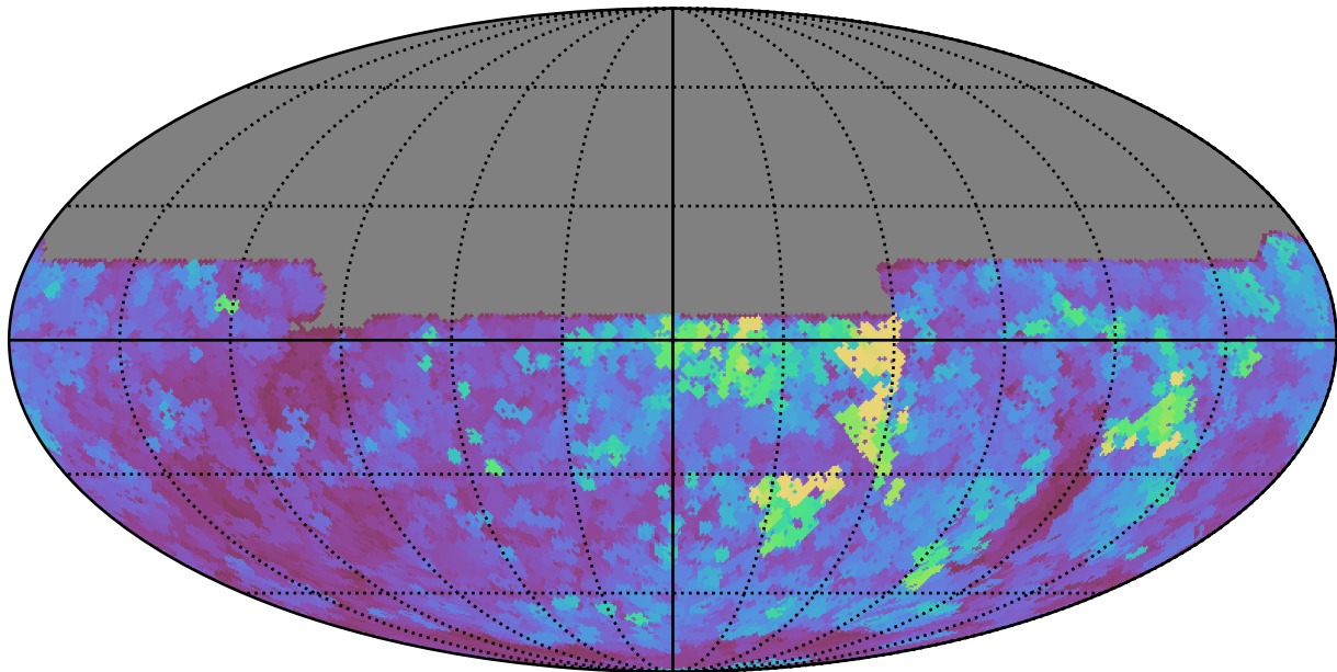
too_elab_r64_d3_griz_v3.4_10yrs All sky y band: Max seeingEff
