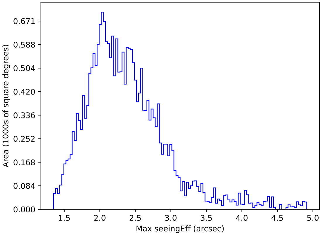
too_elab_r64_d3_griz_v3.4_10yrs All sky y band: Max seeingEff
