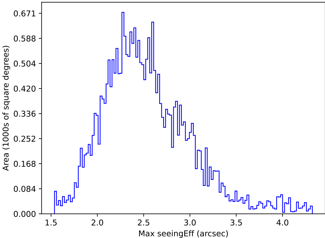
too_elab_r64_d3_griz_v3.4_10yrs All sky r band: Max seeingEff
