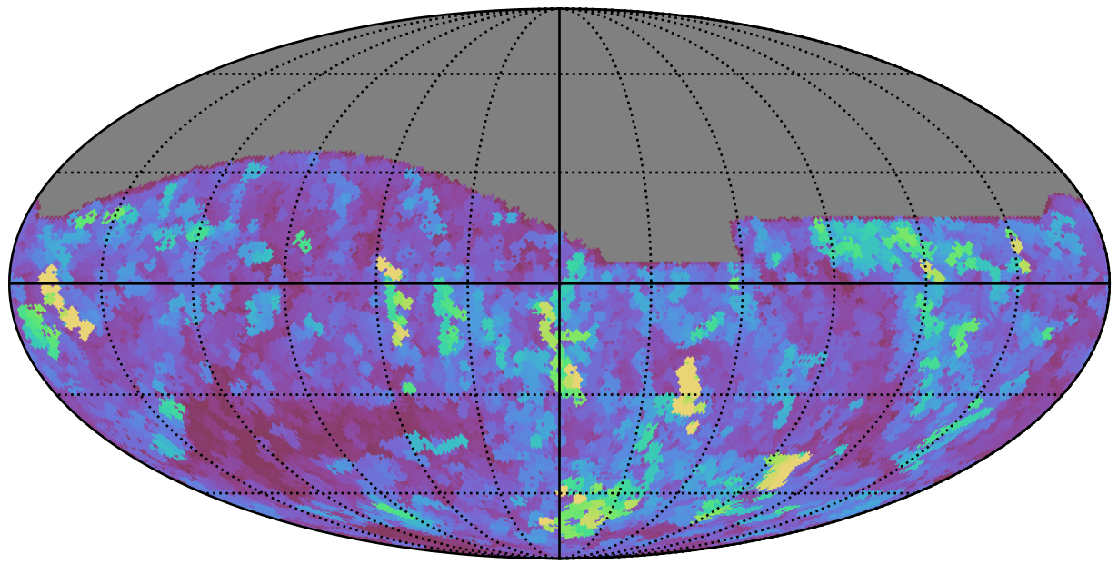
too_elab_r64_d3_griz_v3.4_10yrs All sky i band: Max seeingEff
