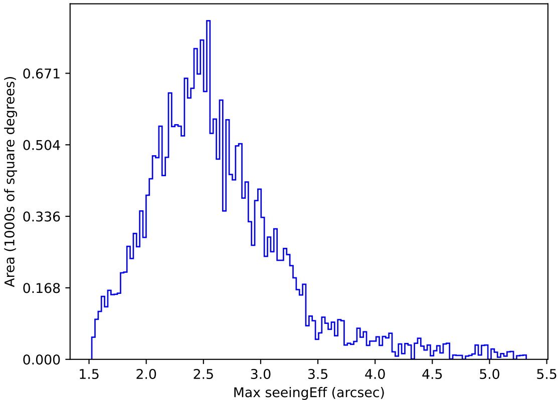
too_elab_r64_d3_griz_v3.4_10yrs All sky i band: Max seeingEff
