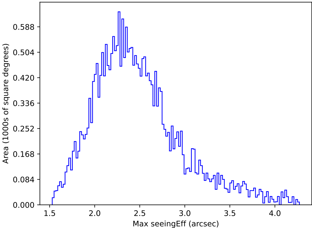
too_elab_r64_d3_griz_v3.4_10yrs All sky g band: Max seeingEff
