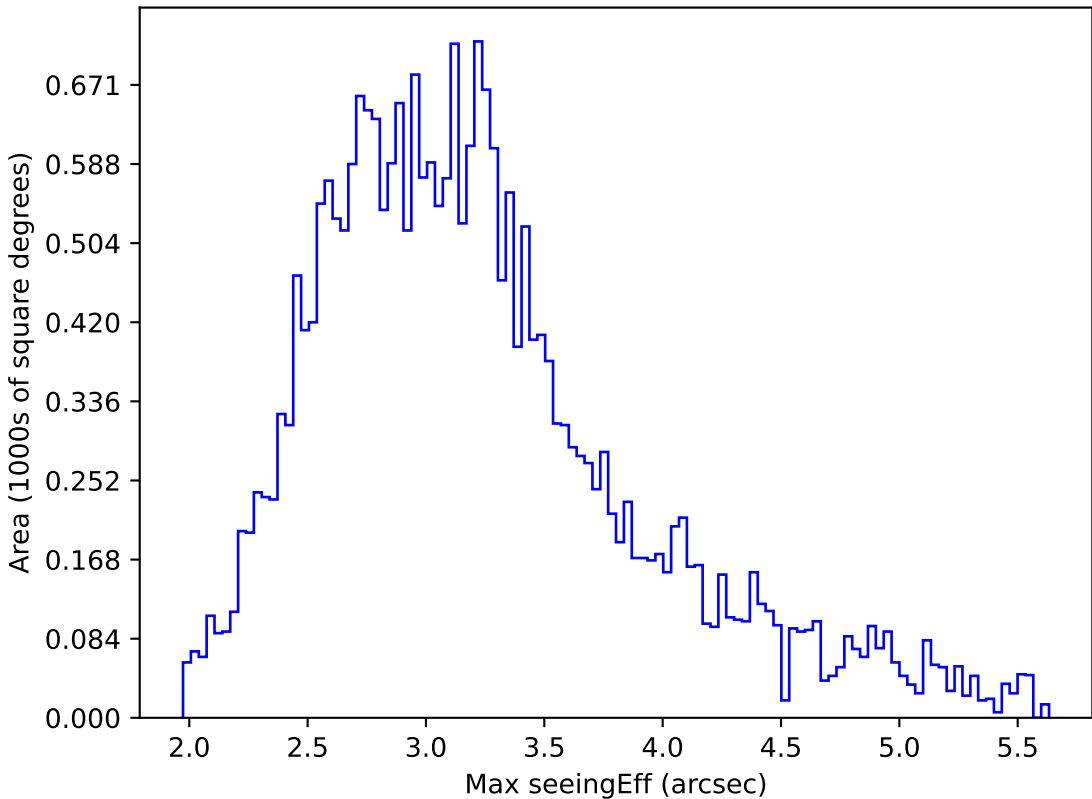
too_elab_r64_d3_griz_v3.4_10yrs All sky all bands: Max seeingEff
