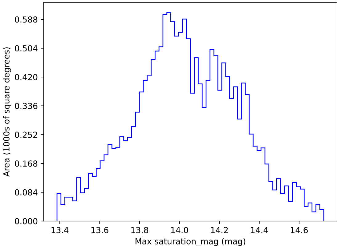
too_elab_r64_d3_griz_v3.4_10yrs WFD u band: Max saturation_mag
