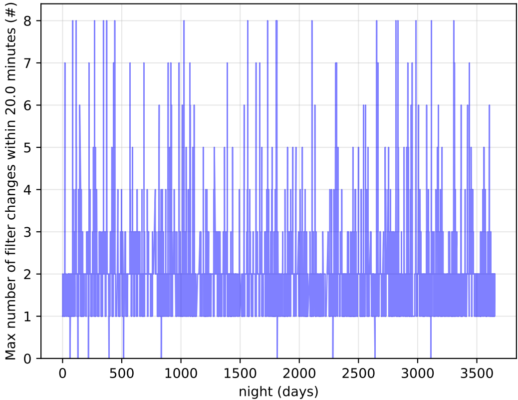
too_elab_r64_d3_griz_v3.4_10yrs Per Night: Max number of filter changes within 20.0 minutes
