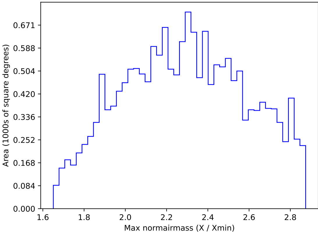
too_elab_r64_d3_griz_v3.4_10yrs WFD z band: Max normairmass
