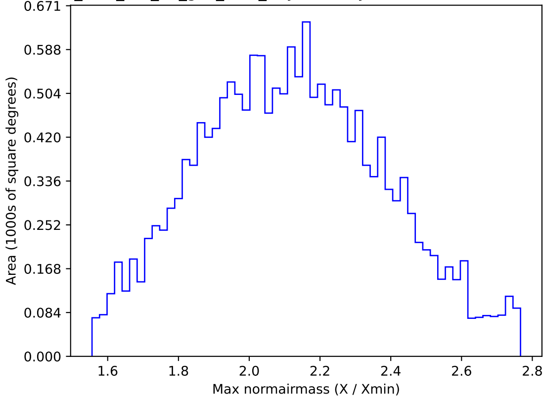
too_elab_r64_d3_griz_v3.4_10yrs WFD y band: Max normairmass
