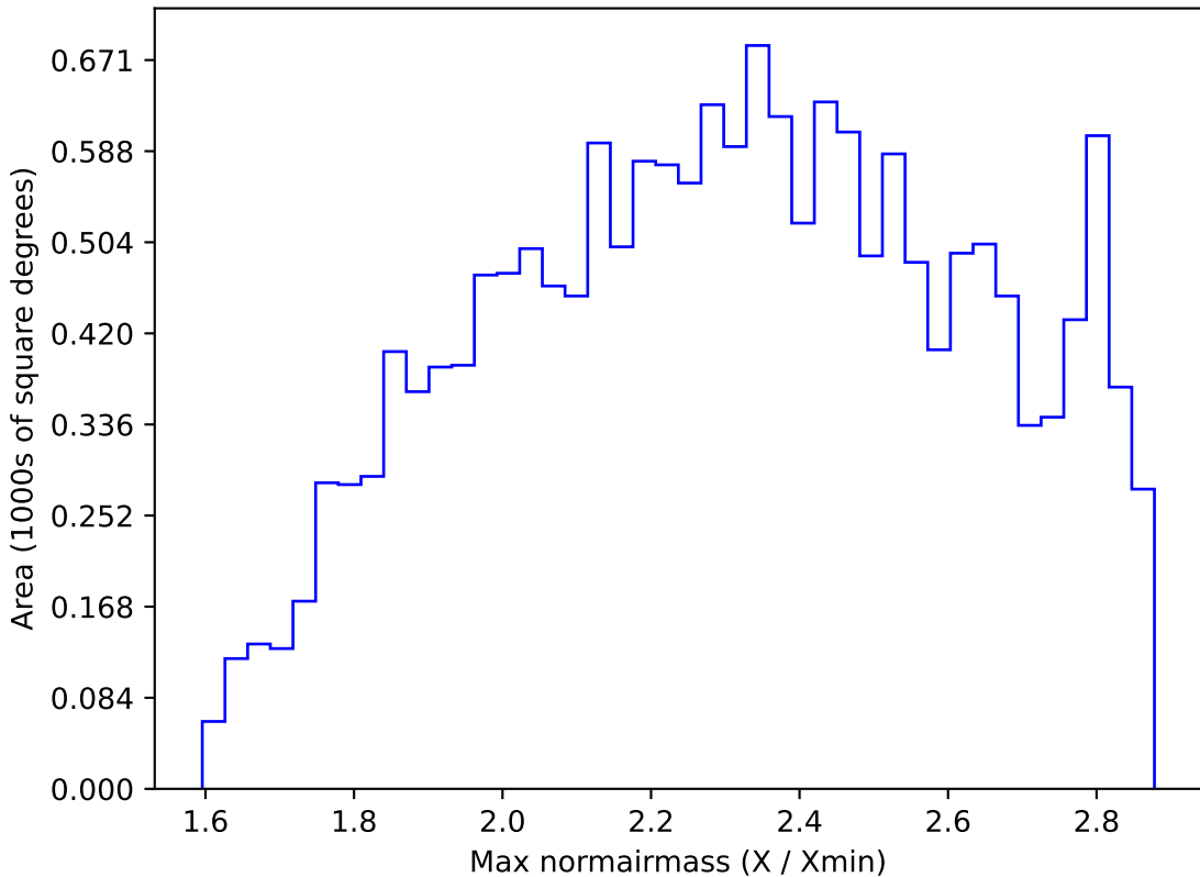
too_elab_r64_d3_griz_v3.4_10yrs WFD i band: Max normairmass
