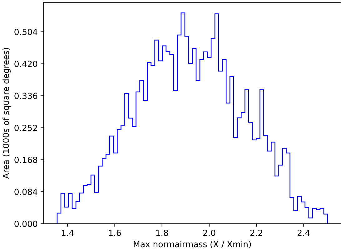
too_elab_r64_d3_griz_v3.4_10yrs WFD g band: Max normairmass
