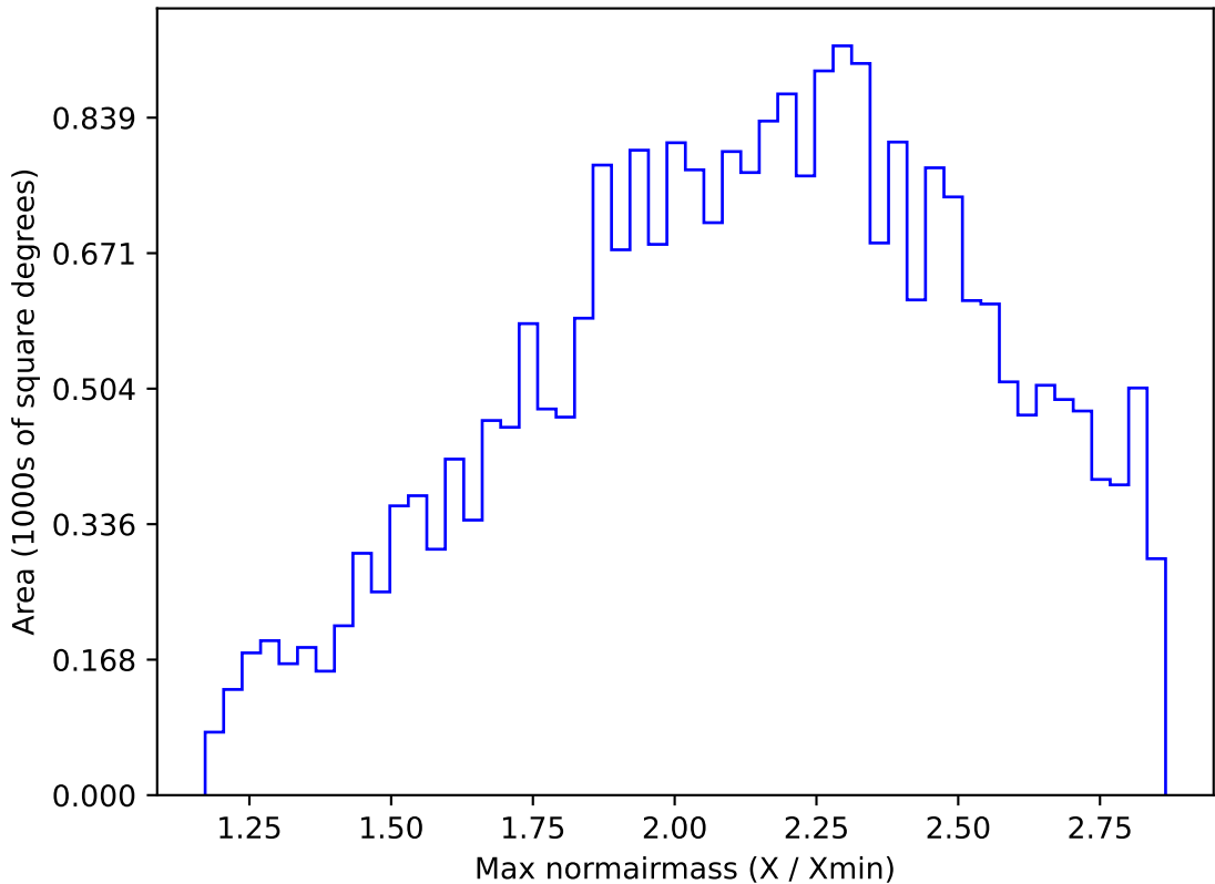
too_elab_r64_d3_griz_v3.4_10yrs All sky z band: Max normairmass
