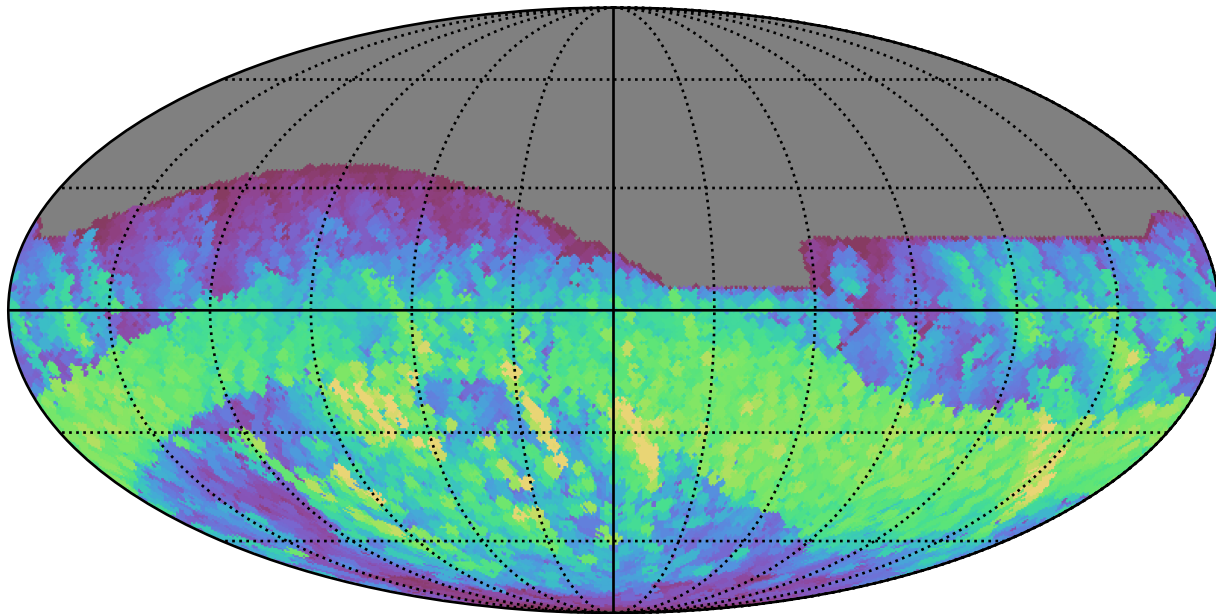
too_elab_r64_d3_griz_v3.4_10yrs All sky r band: Max normairmass
