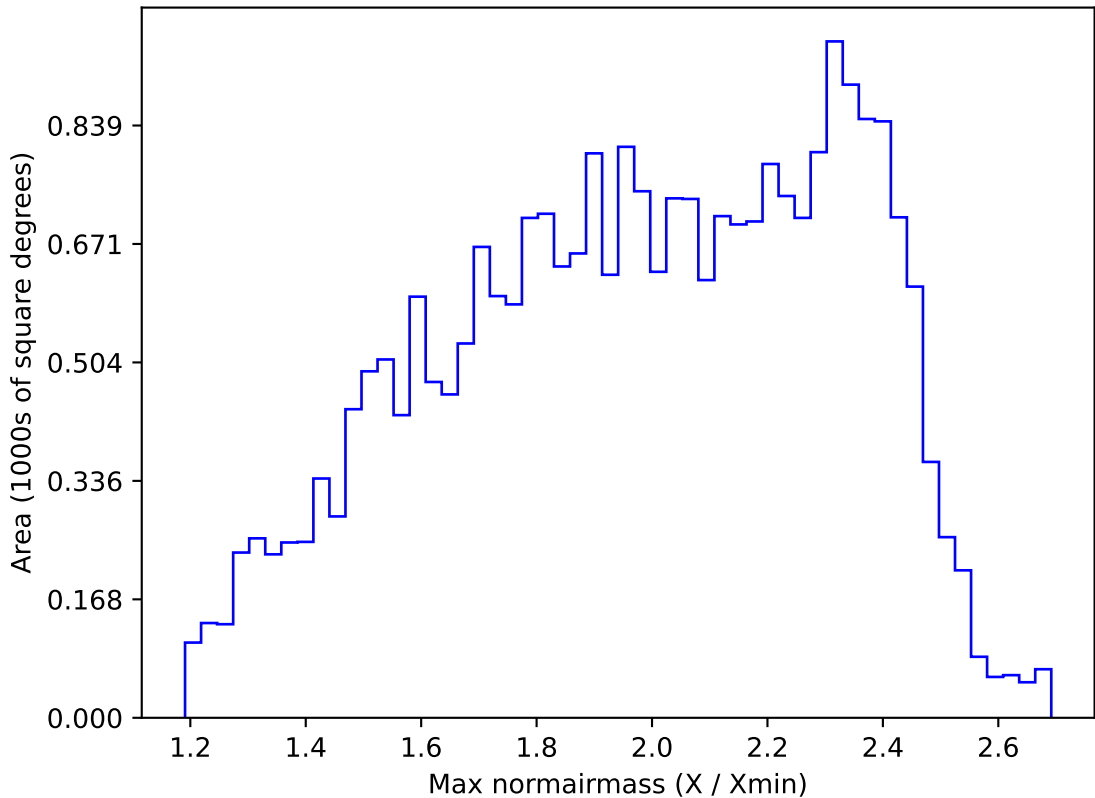
too_elab_r64_d3_griz_v3.4_10yrs All sky r band: Max normairmass
