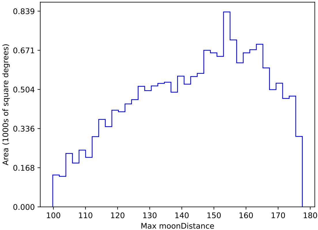
too_elab_r64_d3_griz_v3.4_10yrs WFD y band: Max moonDistance
