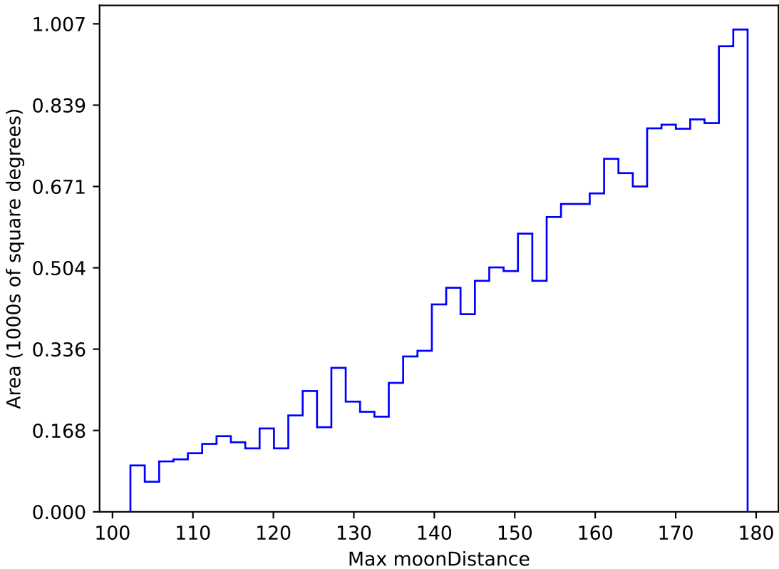
too_elab_r64_d3_griz_v3.4_10yrs WFD u band: Max moonDistance
