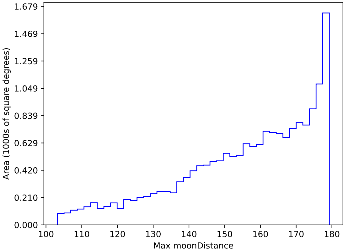
too_elab_r64_d3_griz_v3.4_10yrs WFD r band: Max moonDistance
