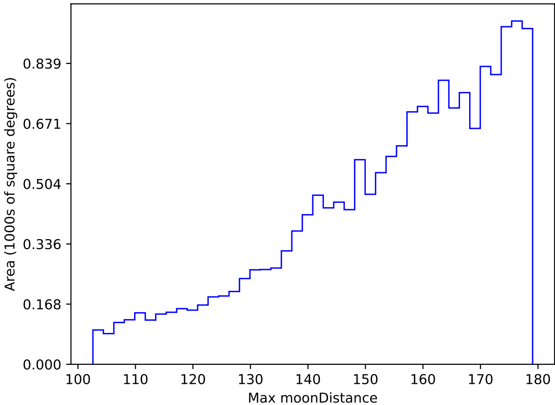
too_elab_r64_d3_griz_v3.4_10yrs WFD g band: Max moonDistance
