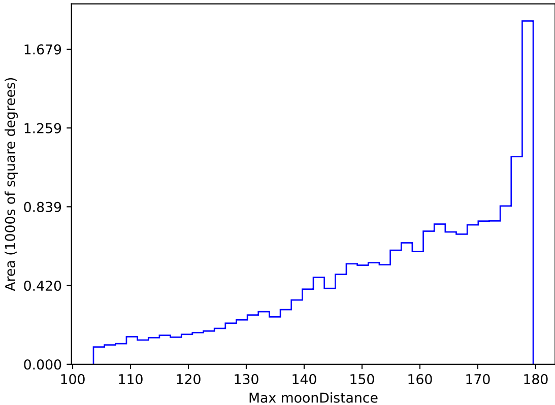
too_elab_r64_d3_griz_v3.4_10yrs WFD all bands: Max moonDistance
