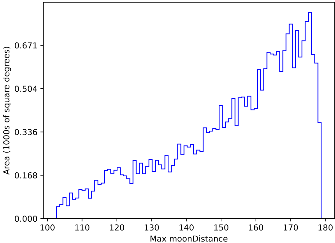
too_elab_r64_d3_griz_v3.4_10yrs All sky z band: Max moonDistance
